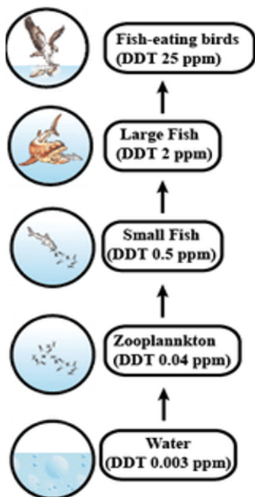
Biomagnification
